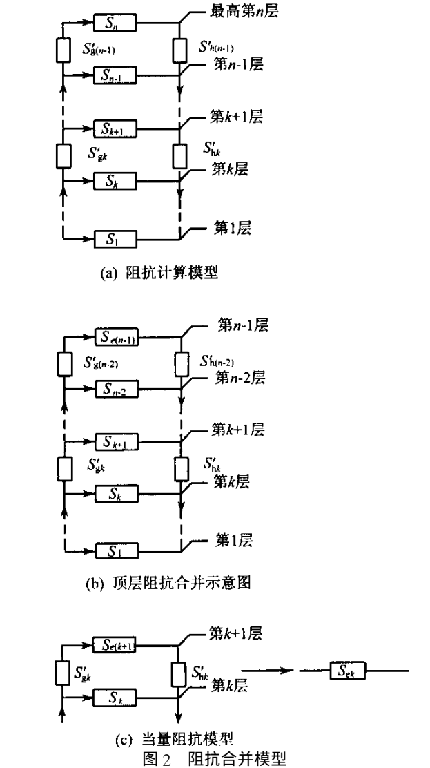
Fig. 2 Model of resistance combination
